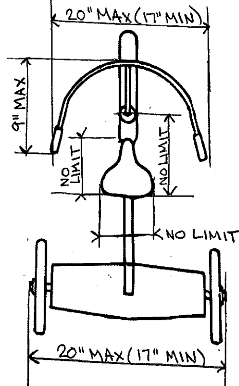
PLAN VIEW
