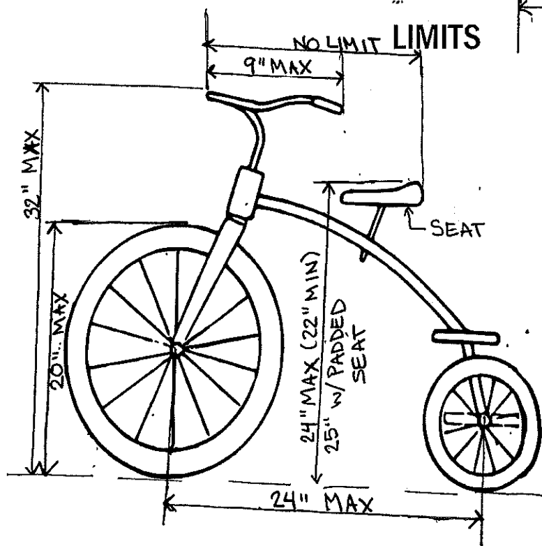
PROFILE VIEW
